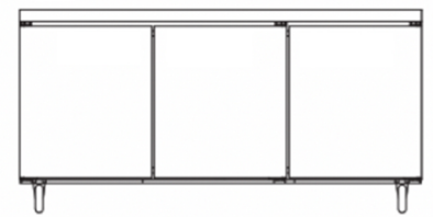
72 FRONT VIEW
