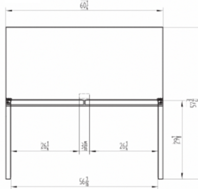
60 FRONT VIEW
