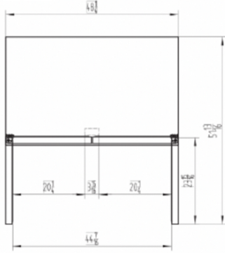
48 TOP VIEW
