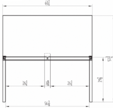
60 FRONT VIEW
