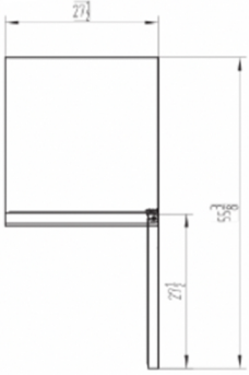
27 TOP VIEW
